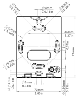
Back plate
